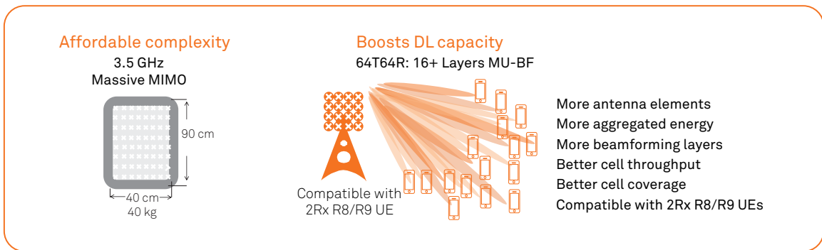
Figure 8: Massive MIMO affordable complexity Source: Huawei
