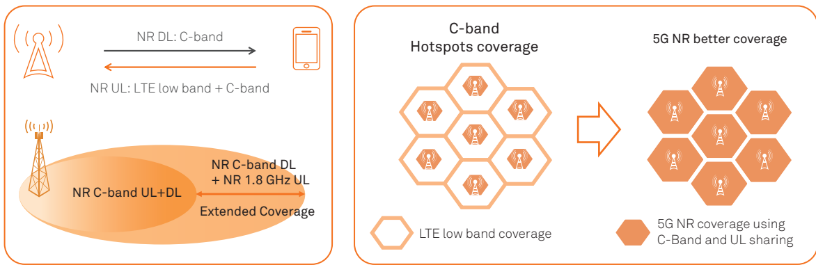
Figure 7: LTE/NR uplink spectrum sharing to extend 5G coverage at higher frequencies (e.g. C-band), accelerate deployment and reduce cost Source: Huawei
